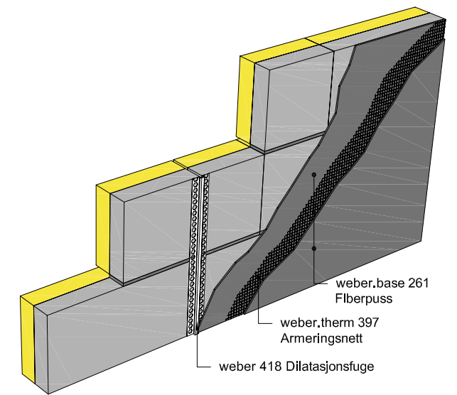
Figur 9.4 webertherm 397 Armeringsnett
