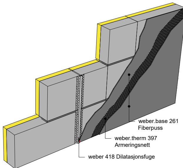
Figur 9.4 webertherm 397 Armeringsnett
