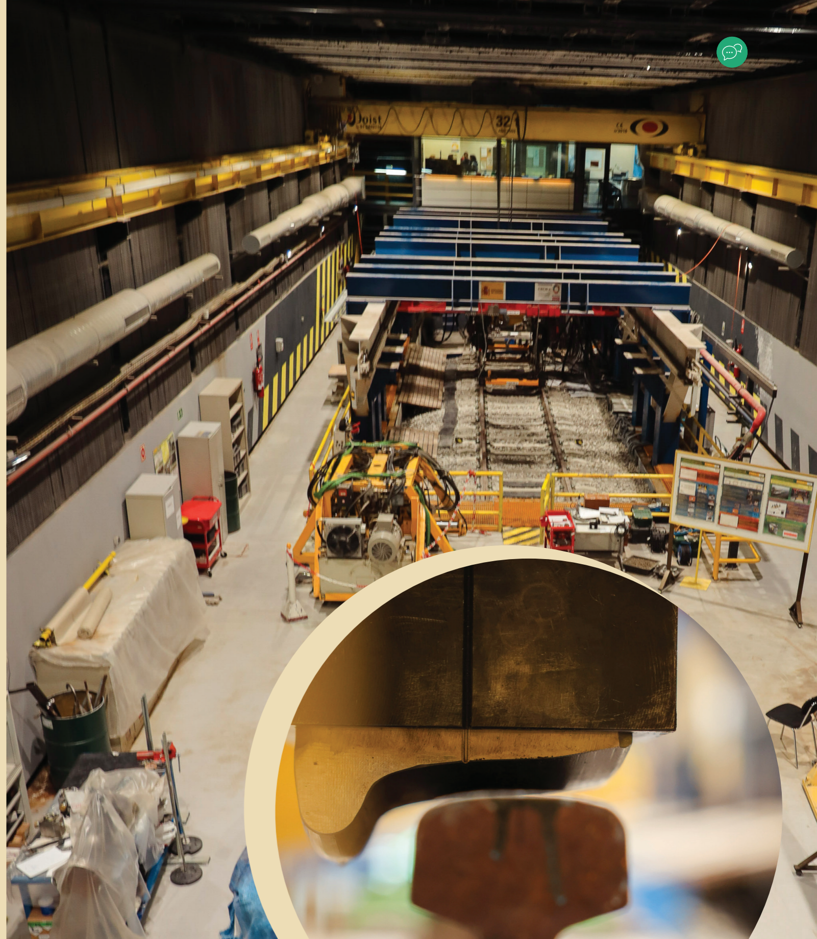
Hydraulic actuators over the railway section
